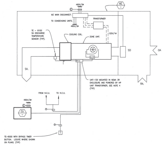
TYPICAL MULTI-ZONE FURNACE SPLIT SYSTEM CONTROL
