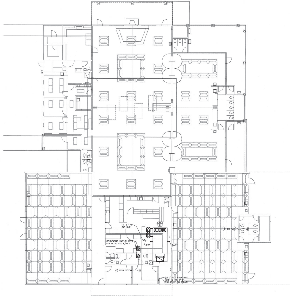
AIR CONDITIONING - BUILDING B - ROOF PLAN SCALE: 1/8" = 1'-0"
