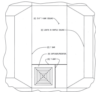
DIFF/REG. ATTACHMENT DETAIL NO SCALE
