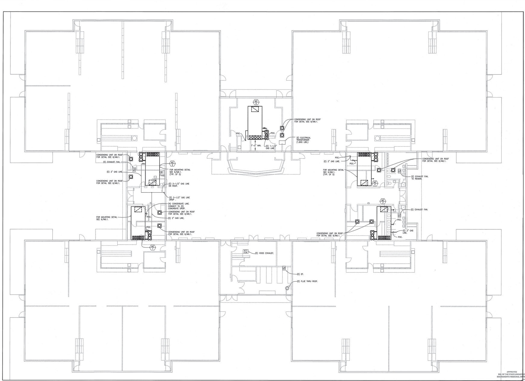
AIR CONDITIONING - BUILDING A - ROOF PLAN SCALE: 1/8"=1'-0"
