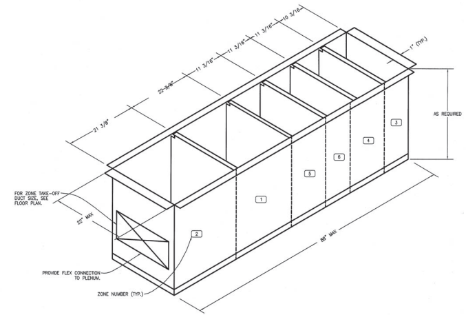
MZ-6 PLENUM DETAIL
