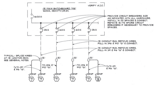
ONE LINE DIAGRAM 480/277 VOLT, 3 PHASE, 4 WIRE NO SCALE
