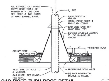
GAS RISER THRU ROOF DETAIL NO SCALE
