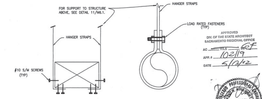
DUCT SUPPORT DETAIL NO SCALE
