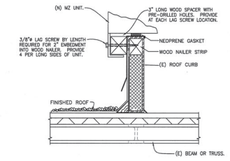
ROOF TOP EQUIPMENT MOUNTING DETAIL NO SCALE
