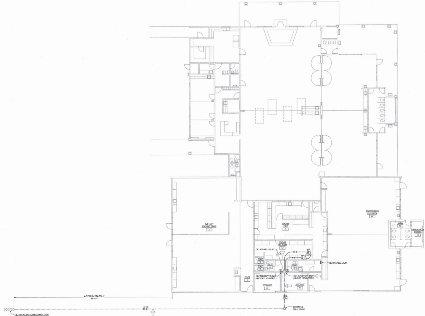
BUILDING-B ELECTRICAL FLOOR PLAN SCALE: 1/8" = 1'-0"
