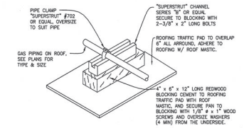
GAS PIPE SUPPORT ON ROOF NO SCALE
