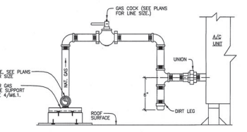
ROOF A/C GAS CONNECTION DETAIL NO SCALE
