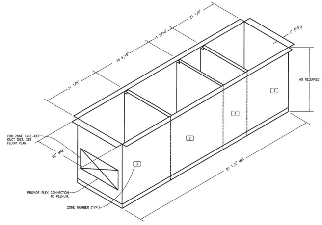
MZ-5 PLENUM DETAIL
