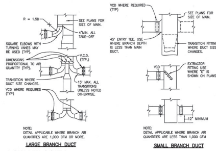
LOW VELOCITY BRANCH DUCT TAKE-OFF DETAIL NO SCALE (LOW VELOCITY 1300 FPM, DUCT SYSTEMS ONLY) NOTE: DUCT SYSTEMS NOT INSTALLED IN ACCORDANCE WITH THIS DETAIL WILL BE REJECTED.
