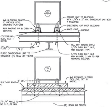
CONDENSING UNIT MOUNTING DETAIL NO SCALE
