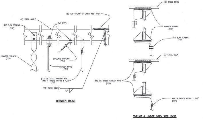
HANGER ROD SUPPORT DETAIL NO SCALE
