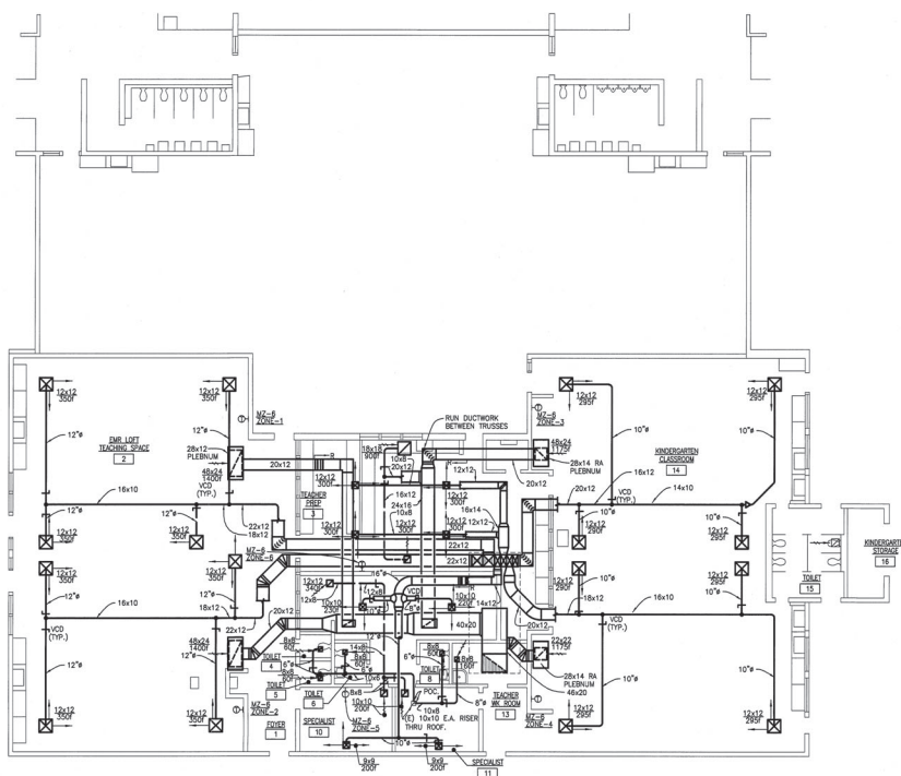
AIR CONDITIONING - BUILDING B - FLOOR PLAN
