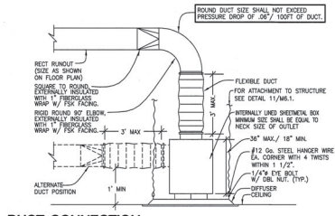
DUCT CONNECTION TO DIFFUSER/ REGISTER DETAIL NO SCALE
