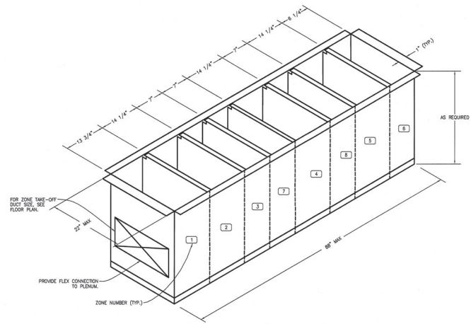
MZ-1, 2, 3, & 4 PLENUM DETAIL
