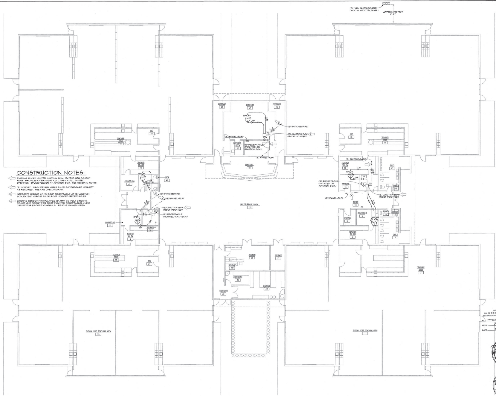
BUILDING-A ELECTRICAL FLOOR PLAN SCALE: 1/8" = 1'-0"
