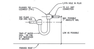
DRAIN PIPE DETAIL NO SCALE
